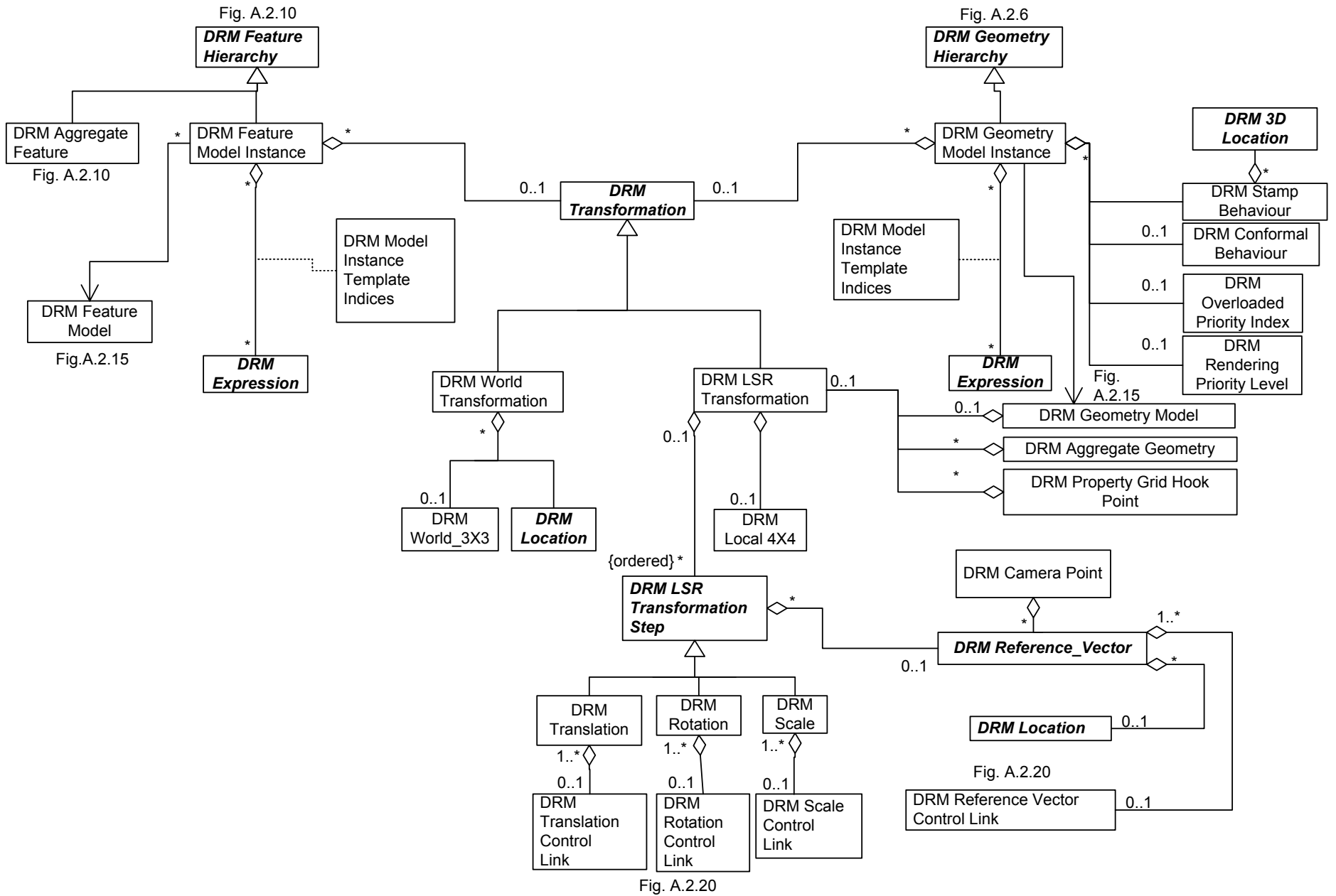
Figure A.2.16 DRM Geometry Model Instance, DRM Feature Model Instance, and DRM Transformation
