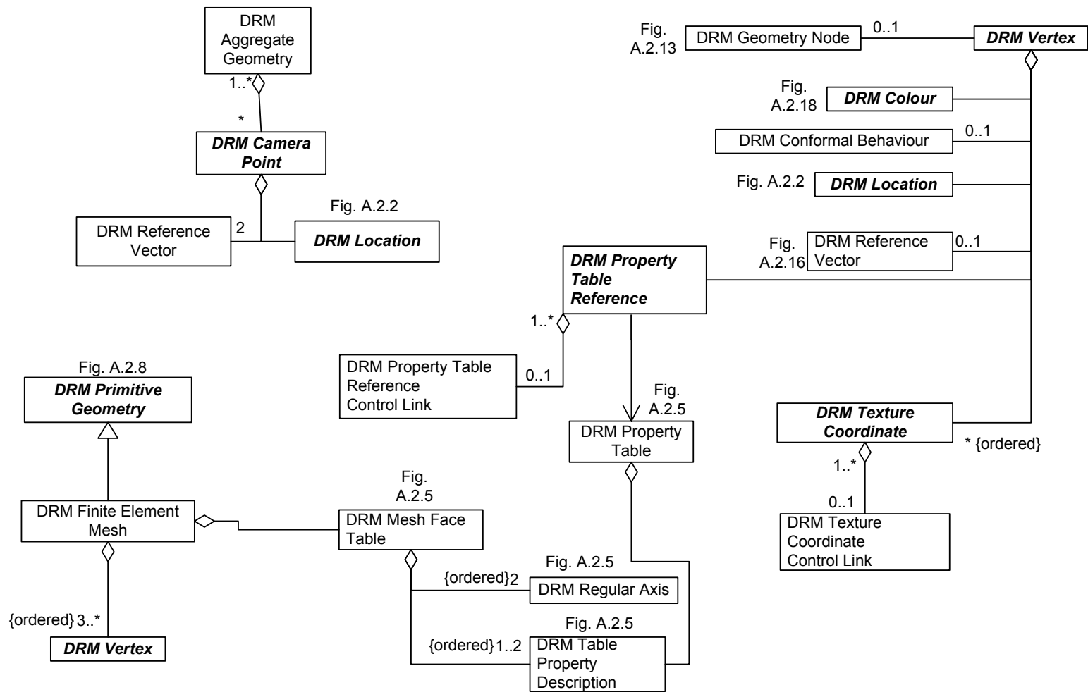
Figure A.2.9 DRM Vertex, DRM Finite Element Mesh, and DRM Camera Point
