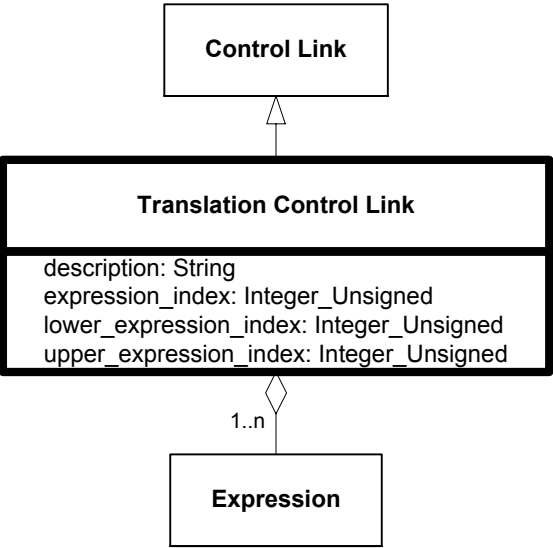
Figure 6.335—DRM_Translation_Control_Link
