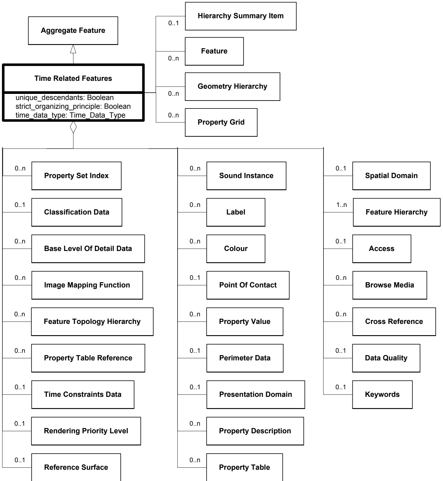
Figure 6.327—DRM_Time_Related_Features
