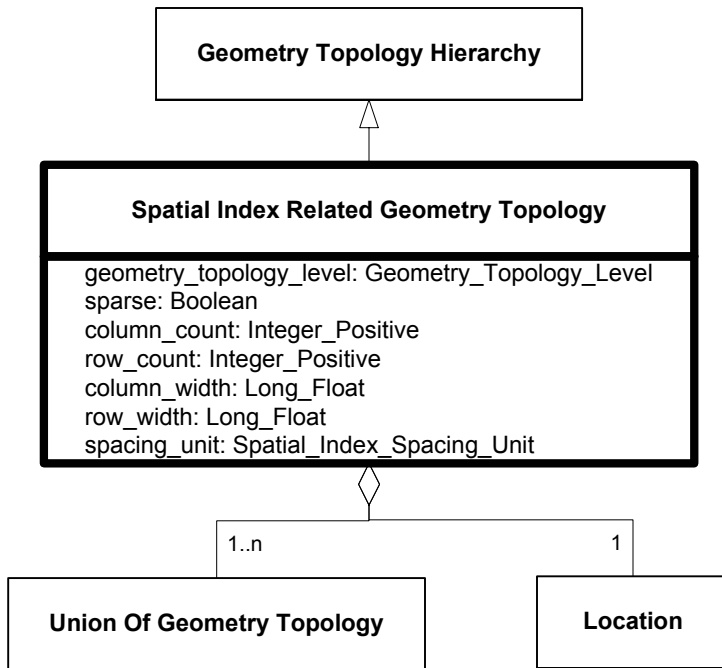
Figure 6.296—DRM_Spatial_Index_Related_Geometry_Topology
