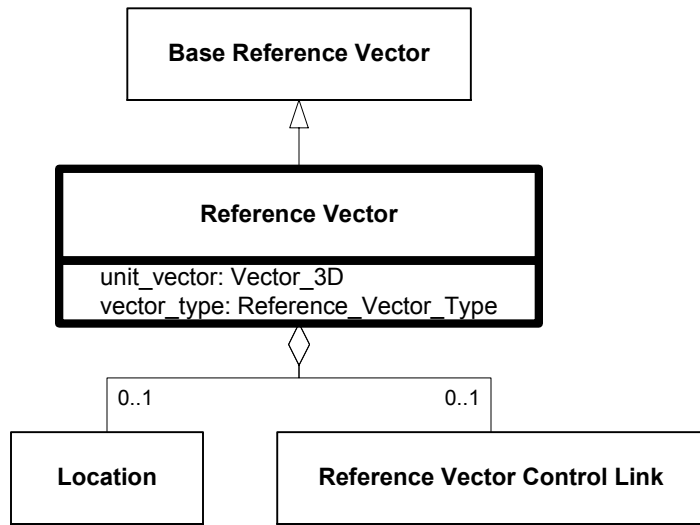
Figure 6.253—DRM_Reference_Vector
