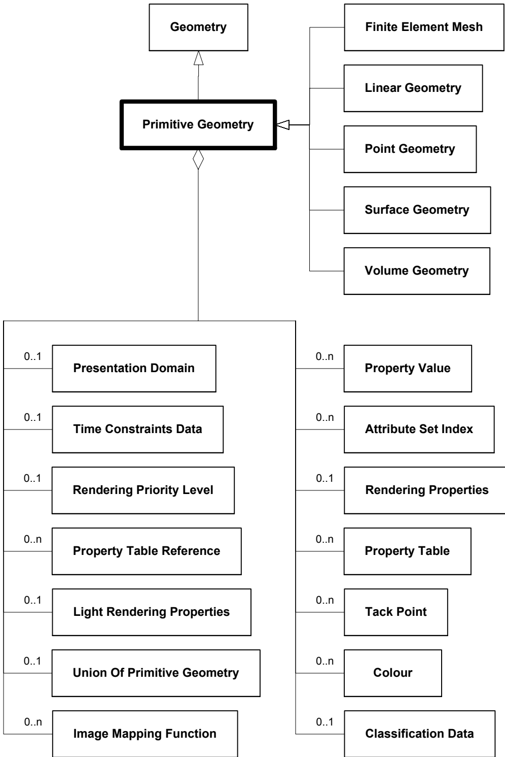
Figure 6.211—DRM_Primitive_Geometry
