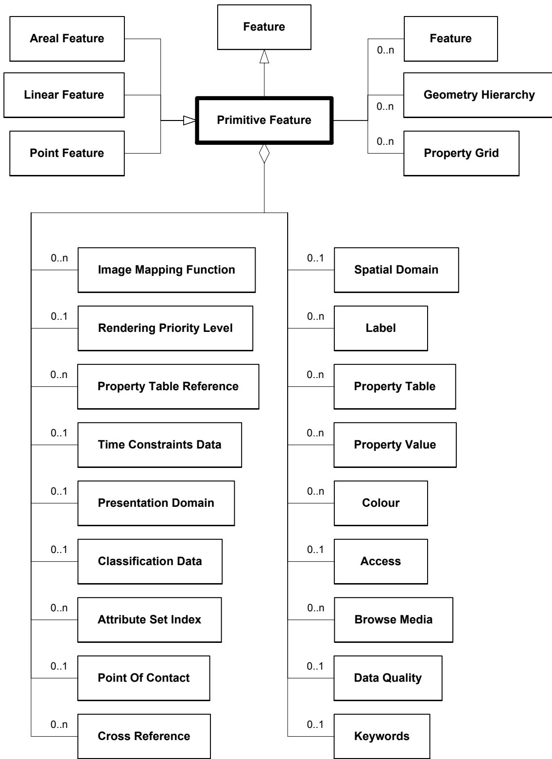
Figure 6.210—DRM_Primitive_Feature
