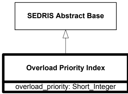
Figure 6.193—DRM_Overload_Priority_Index
