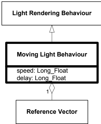
Figure 6.185—DRM_Moving_Light_Behaviour
