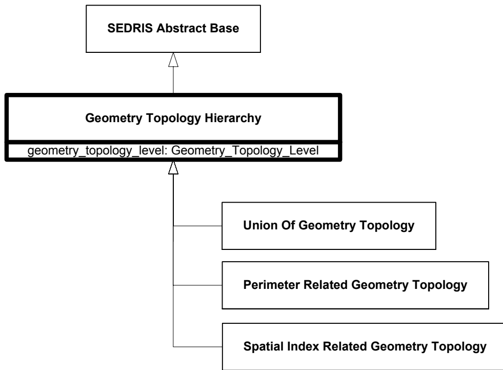
Figure 6.116—DRM_Geometry_Topology_Hierarchy
