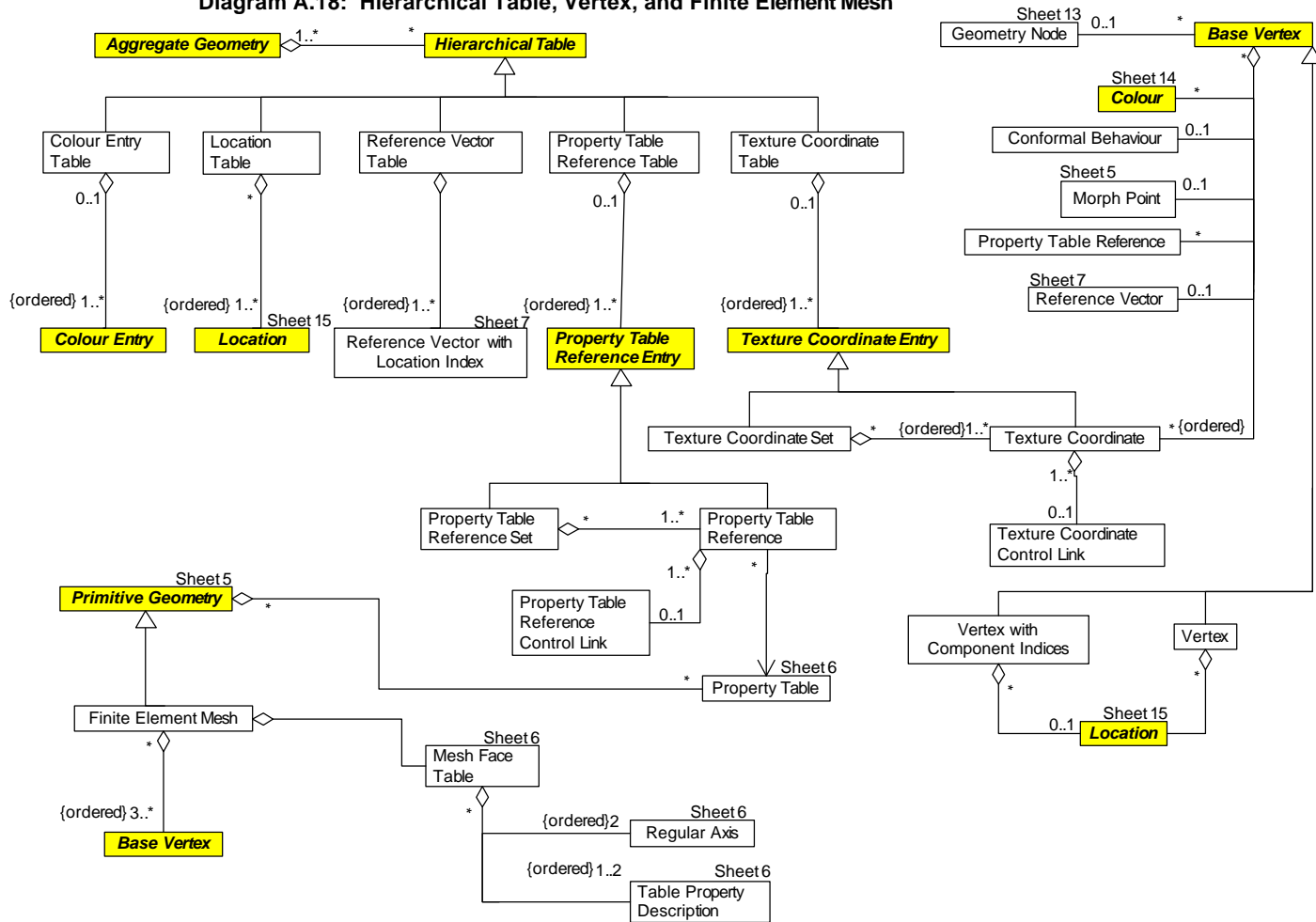
Diagram A.18: Hierarchical Table, Vertex, and Finite Element Mesh
