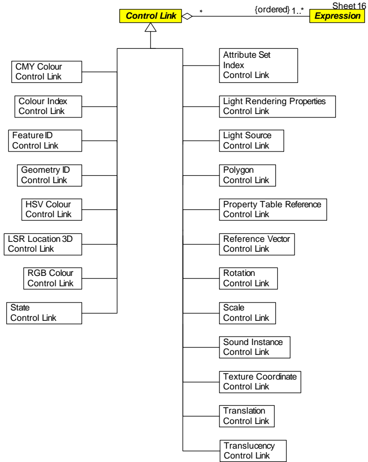
Diagram A.17: Control Link Subclasses
