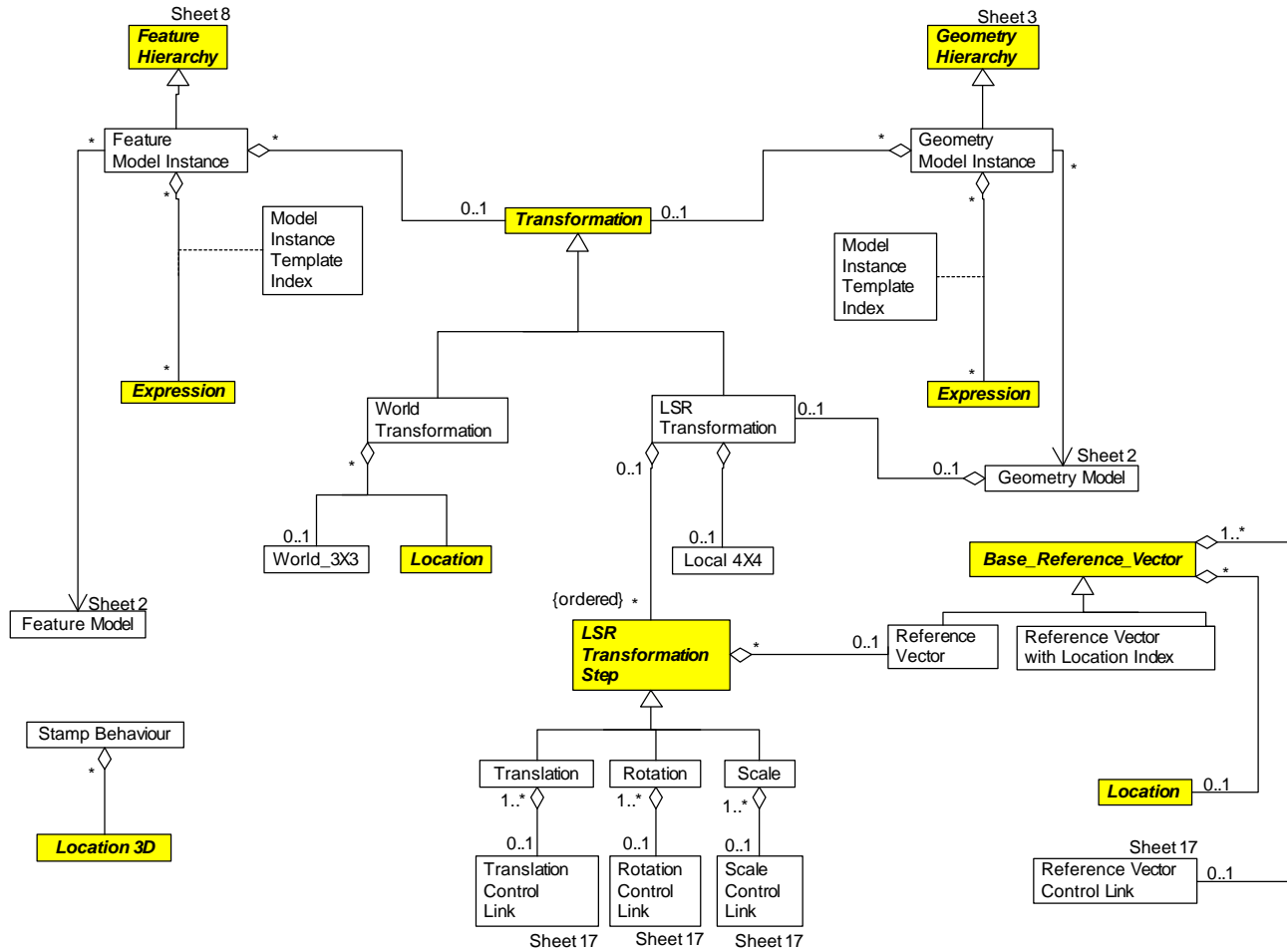
Diagram A.7: Geometry Model Instance, Feature Model Instance, and Transformation
