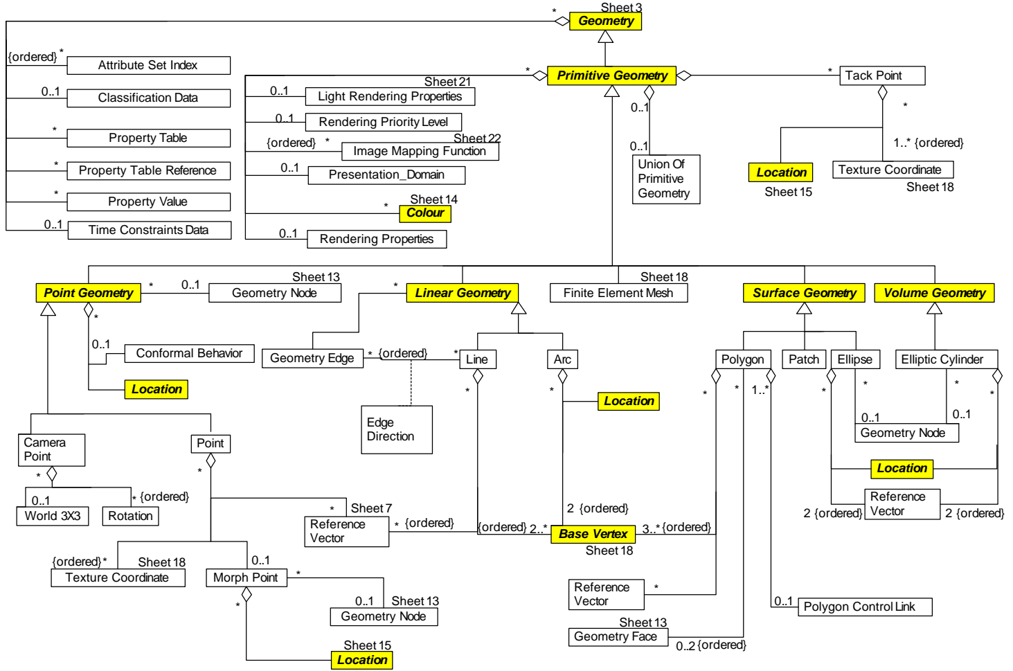
Diagram A.5: Primitive Geometry
