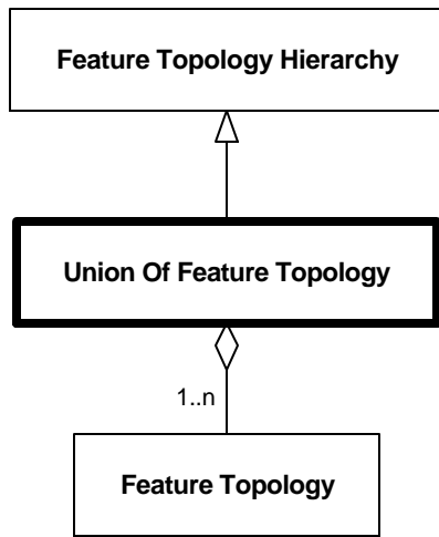
Diagram 6.307--DRM_Union_Of_Feature_Topology
