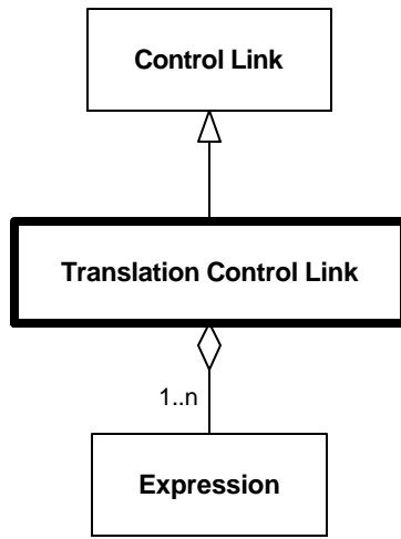
Diagram 6.301--DRM_Translation_Control_Link
