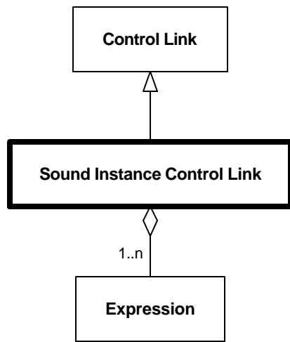
Diagram 6.260--DRM_Sound_Instance_Control_Link
