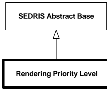
Diagram 6.236--DRM_Rendering_Priority_Level
