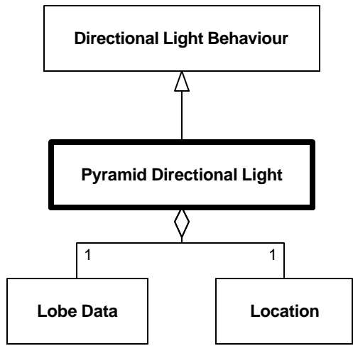
Diagram 6.222--DRM_Pyramid_Directional_Light
