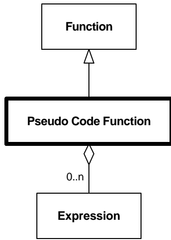
Diagram 6.221--DRM_Pseudo_Code_Function
