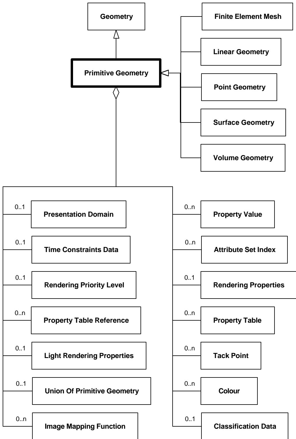
Diagram 6.205--DRM_Primitive_Geometry
