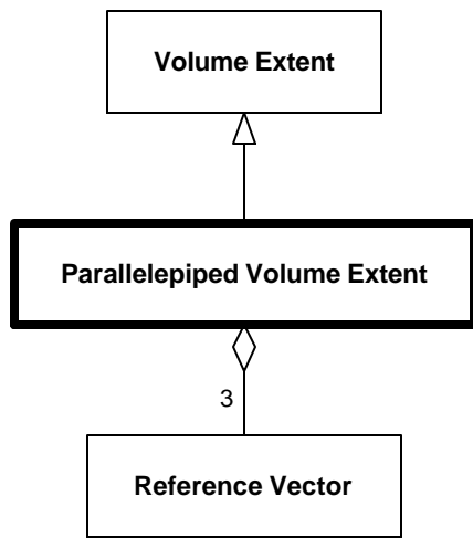
Diagram 6.188--DRM_Parallelepiped_Volume_Extent
