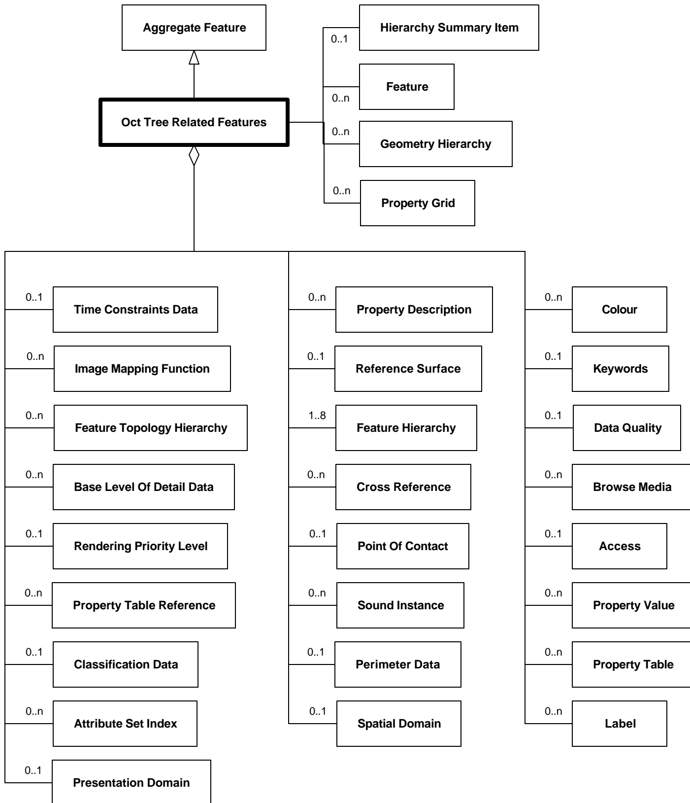
Diagram 6.184--DRM_Oct_Tree_Related_Features
