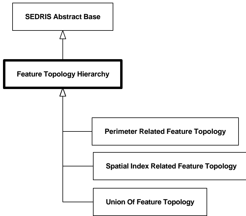
Diagram 6.102—DRM_Feature_Topology_Hierarchy
