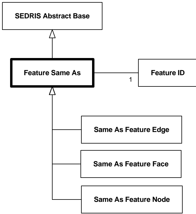
Diagram 6.100—DRM_Feature_Same_As
