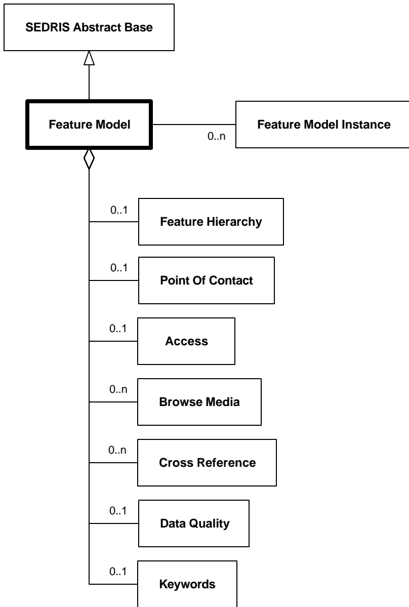
Diagram 6.97—DRM_Feature_Model
