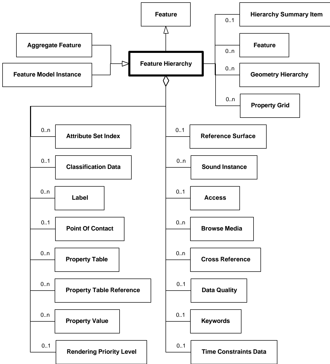
Diagram 6.94—DRM_Feature_Hierarchy
