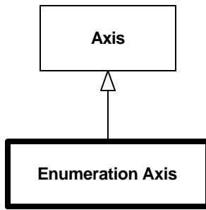
Diagram 6.83—DRM_Enumeration_Axis
