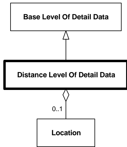
Diagram 6.75—DRM_Distance_Level_Of_Detail_Data
