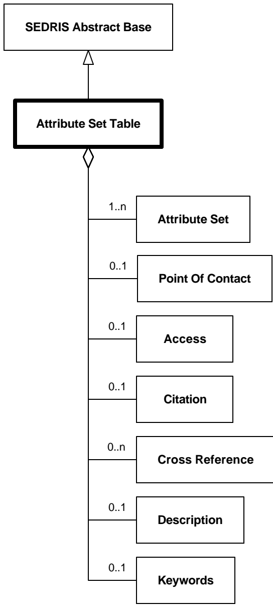
Diagram 6.23--DRM_Attribute_Set_Table
