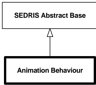
Diagram 6.12--DRM_Animation_Behaviour
