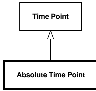
Diagram 6.2--DRM_Absolute_Time_Point
